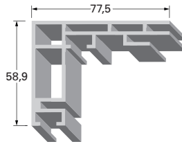
LED frame 77,5 (LED 77,5) 1,86 kg/m
