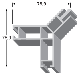
frame Cube Eckstrebe (Cube vertical) 1,99 kg/m
