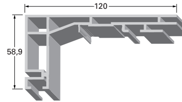
LED frame 120 (LED 120) 2,34 kg/m
