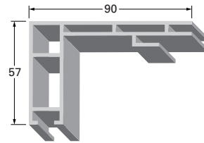
LED frame 90 (LED 90) 1,88 kg/m
