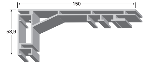
LED frame 150 (LK 1) 2,79 kg/m
