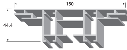
LED frame 150 D (LED 150) 3,03 kg/m
