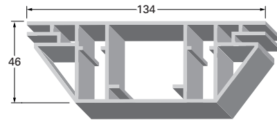
LED frame 134 D (LED EdgeLit Double) 3,2 kg/m
