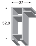
frame 32 (System 1) 1,02 kg/m
