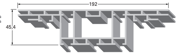
LED frame 192 D (LK 2) 4,01 kg/m
