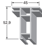
frame 45 D (System 3) 1,16 kg/m
